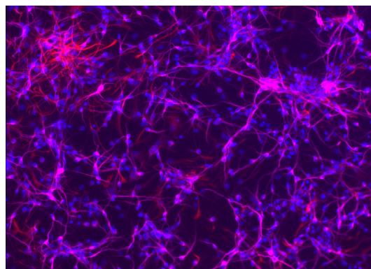
A photomicrograph of NSCs treated with 10 \mu\text{M} BaP from the study. The neurons and glia show the development of the projections through which developing neural cells communicate with each other. The blue dots indicate cell nuclei, red indicates glia, and purple indicates neurons. (Photo courtesy of Theodore Slotkin)
