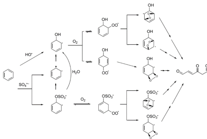
The researchers illustrated the process by which 4-oxo-2-hexenedial, a toxic breakdown product of benzene, is formed during chemical oxidation. (Image from Van Buren et al., 2020, Environ Sci Technol)
