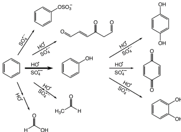
A simplified representation of the many chemical reactions and byproducts detected from the oxidation of benzene by hydrogen peroxide (HO) or persulfate (SO 4 ). (Image from Van Buren et al., 2020, Environ Sci Technol)
