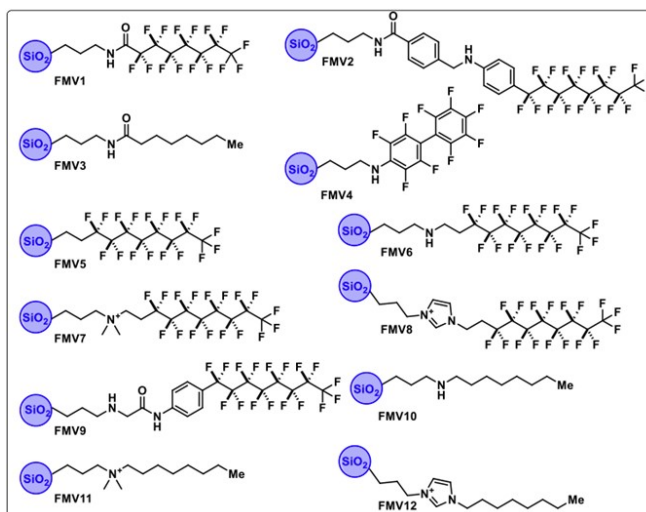
The 12 Fluor Mop materials made of silica (SiO 2 ) and fluorine were similar in structure but had minor changes in their components, such as the addition of ammonia derivatives. (Image courtesy of Singh et al., 2023)
