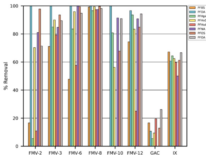
Results showing the ability of six Fluor Mop materials, granular activated carbon (GAC), and ion exchange resins (IX) to remove eight different PFAS compounds.
