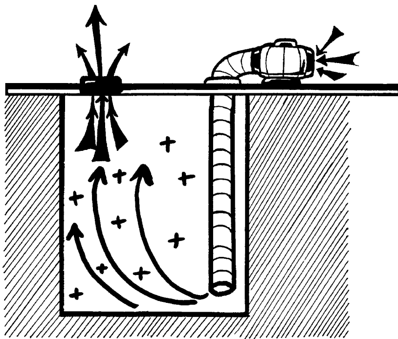
Addition of Duct Work to Avoid Short Circuting
